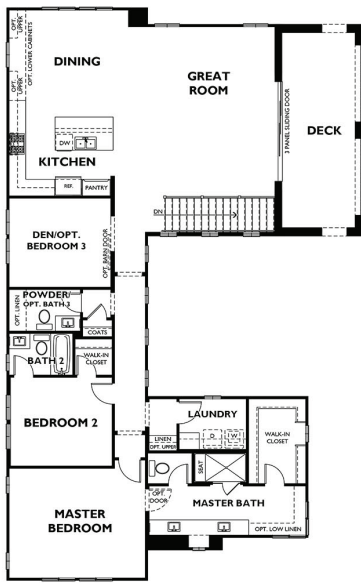
2nd Floor Plan Elevation A
