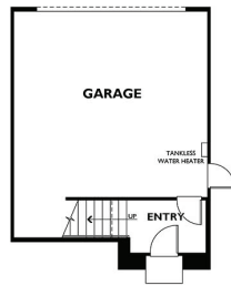
1st Floor Plan Elevation A
